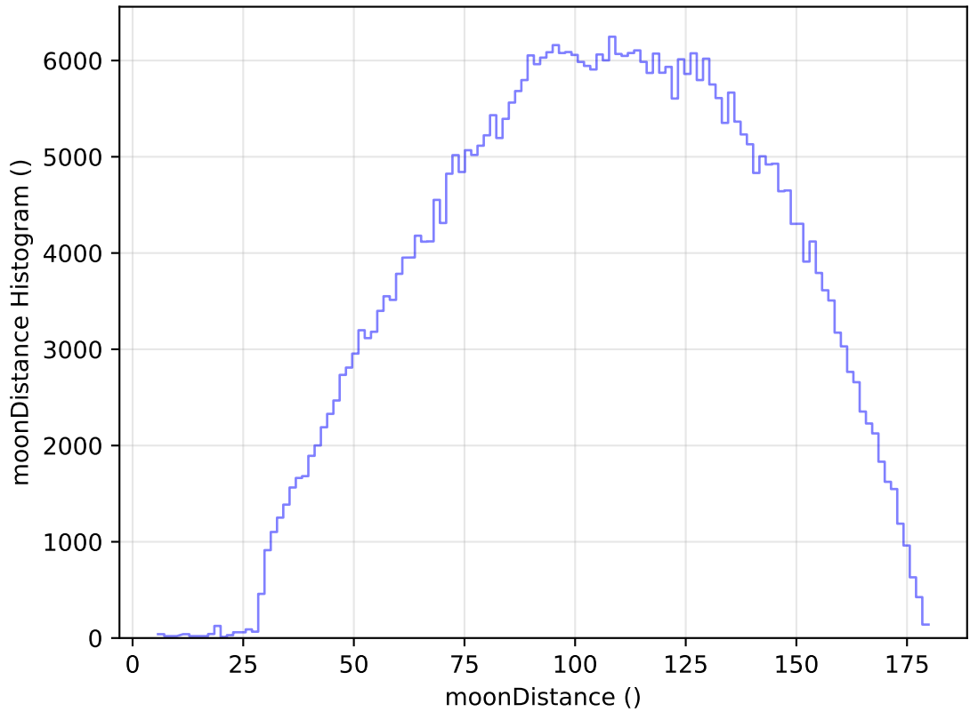
internal_u_expt60_nscale1.5v3.4_10yrs WFD r band: moonDistance Histogram
