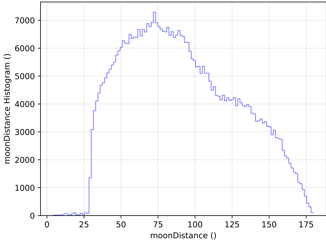
internal_u_expt60_nscale1.5v3.4_10yrs WFD i band: moonDistance Histogram
