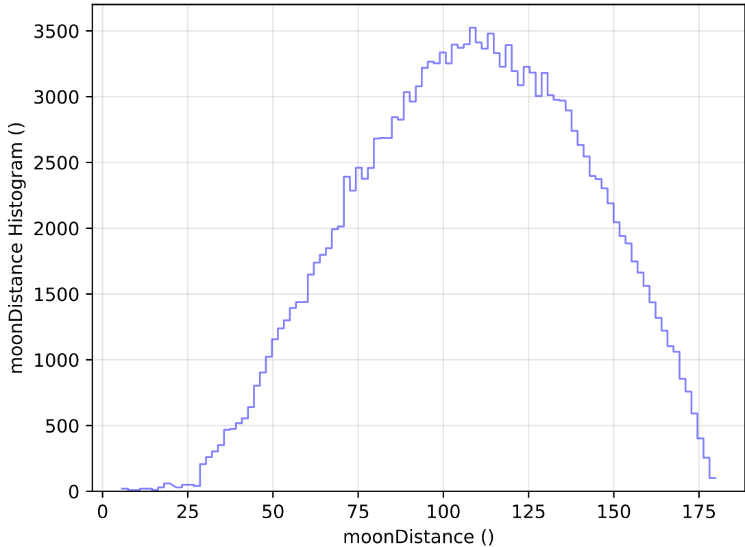
internal_u_expt60_nscale1.5v3.4_10yrs WFD g band: moonDistance Histogram
