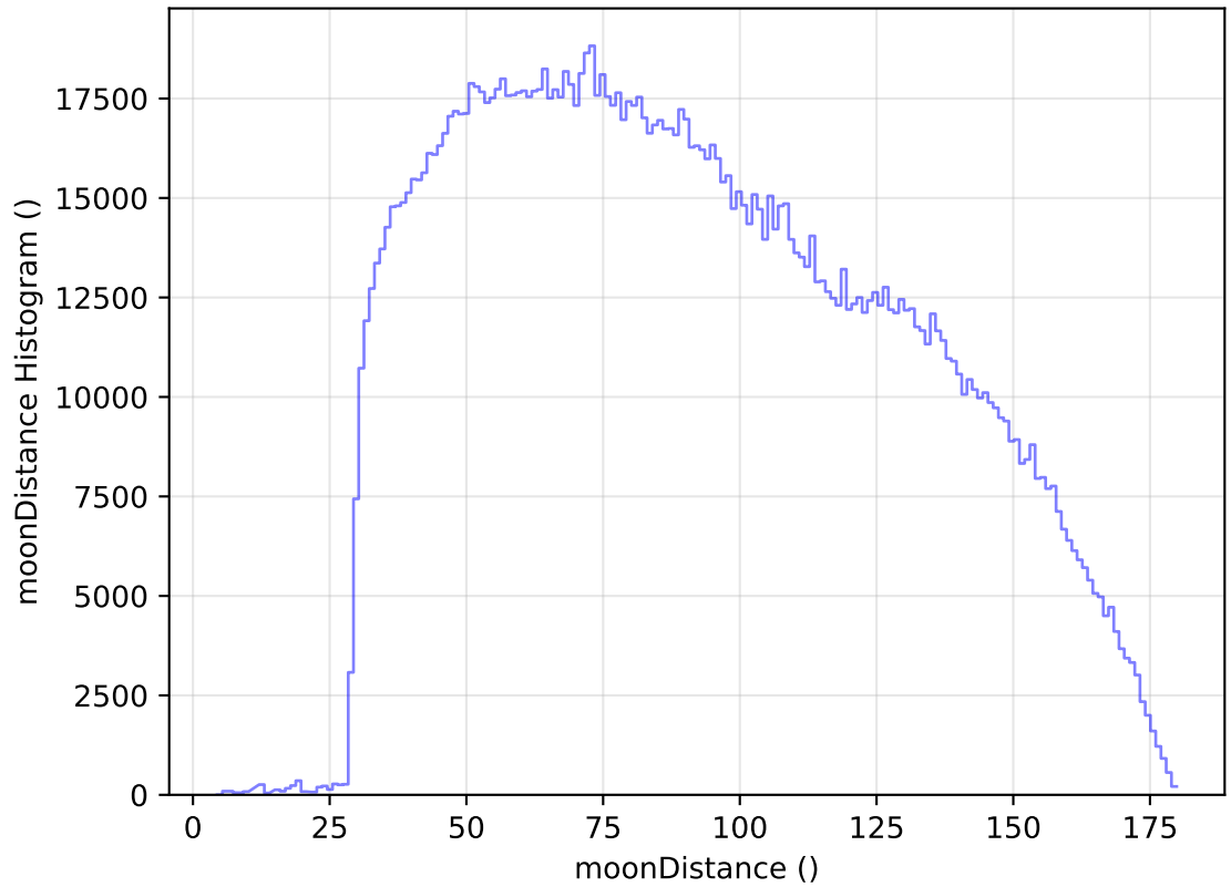
internal_u_expt60_nscale1.5v3.4_10yrs WFD all bands: moonDistance Histogram
