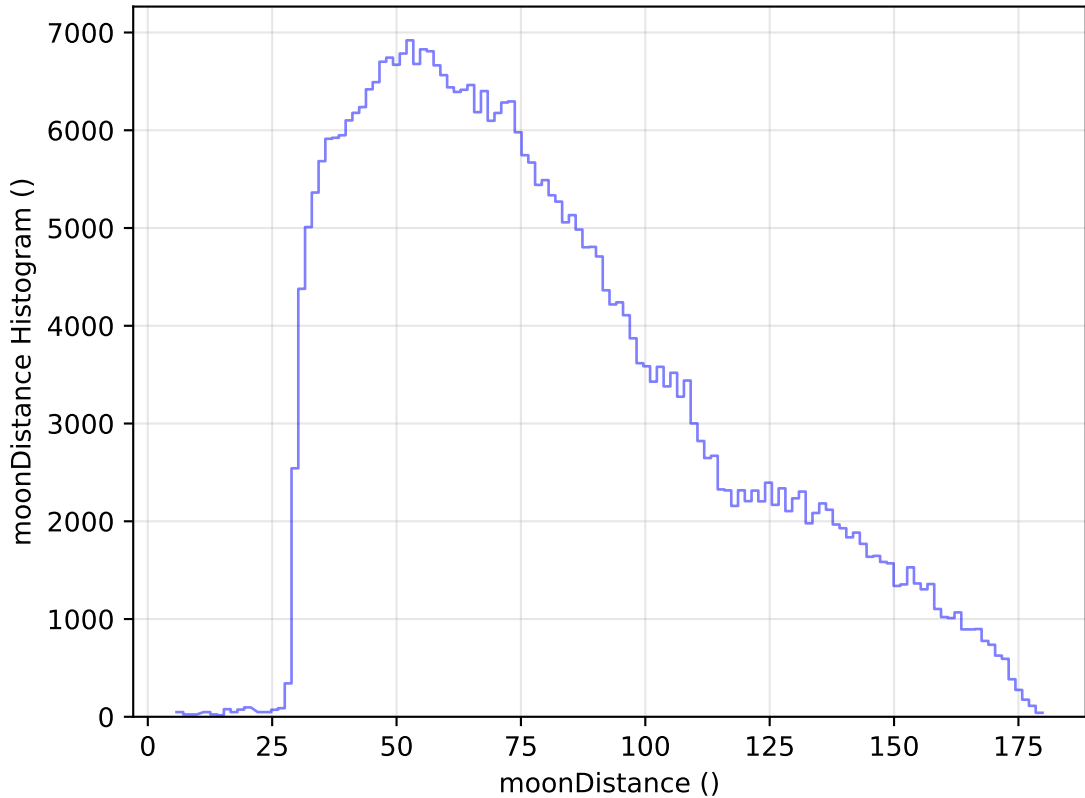
internal_u_expt60_nscale1.5v3.4_10yrs All sky z band: moonDistance Histogram
