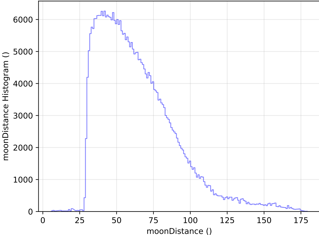
internal_u_expt60_nscale1.5v3.4_10yrs All sky y band: moonDistance Histogram
