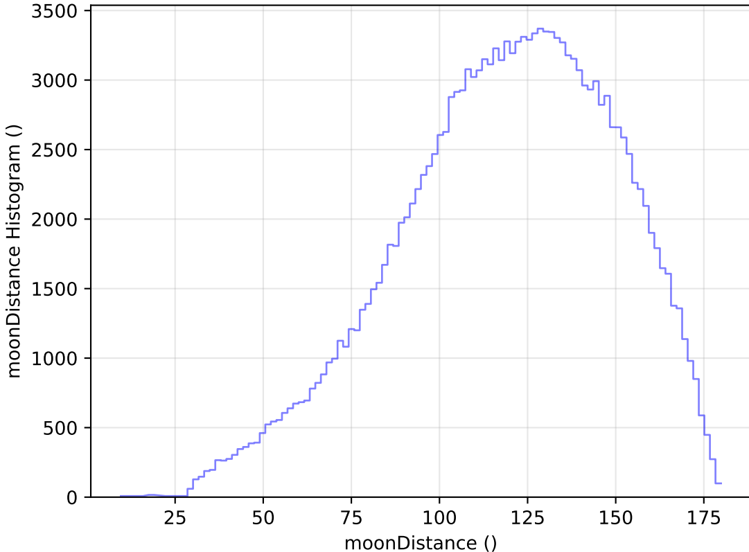
internal_u_expt60_nscale1.5v3.4_10yrs All sky u band: moonDistance Histogram
