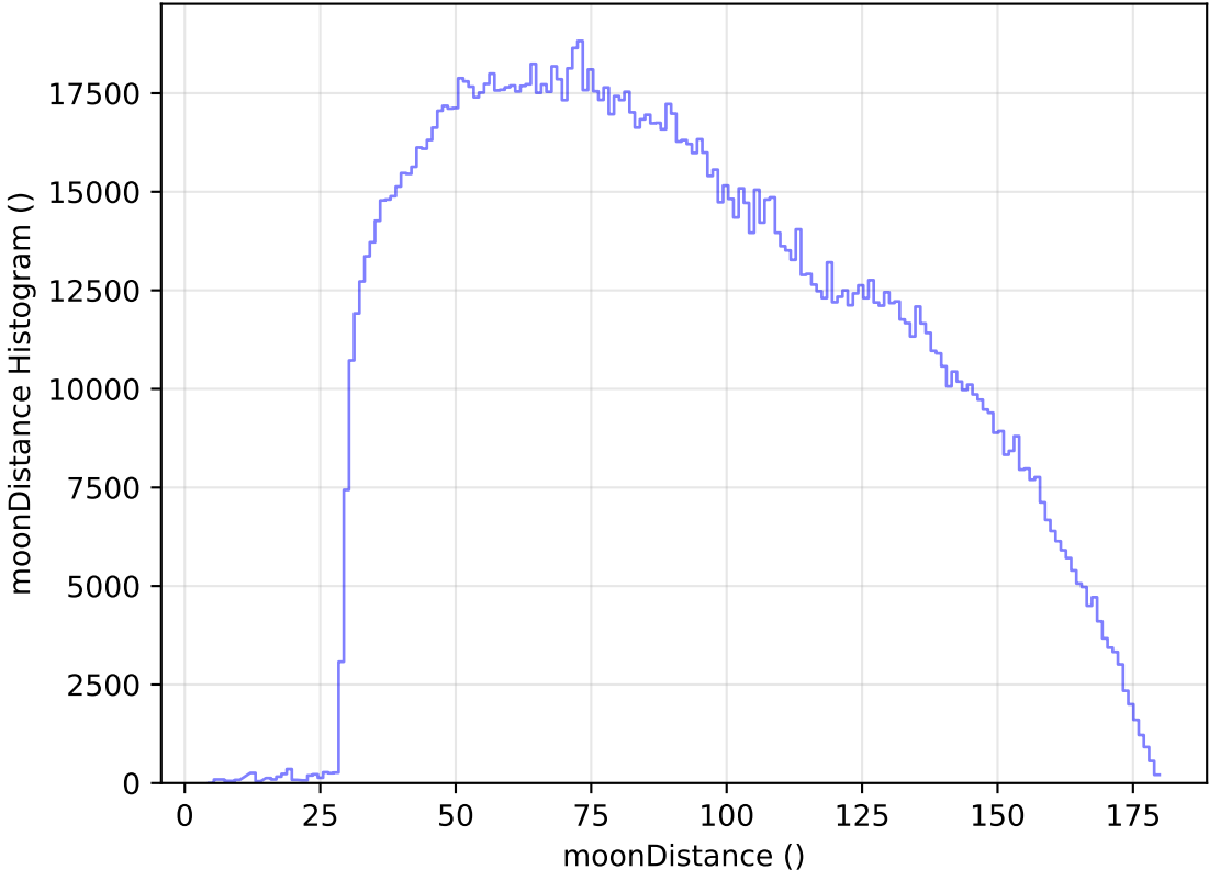
internal_u_expt60_nscale1.5v3.4_10yrs All sky all bands: moonDistance Histogram
