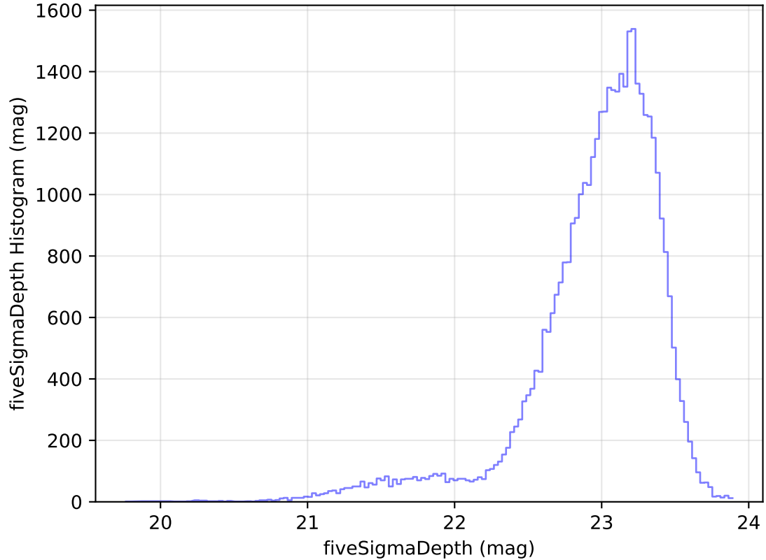
internal_u_expt60_nscale1.5v3.4_10yrs Yr 1 z band: fiveSigmaDepth Histogram
