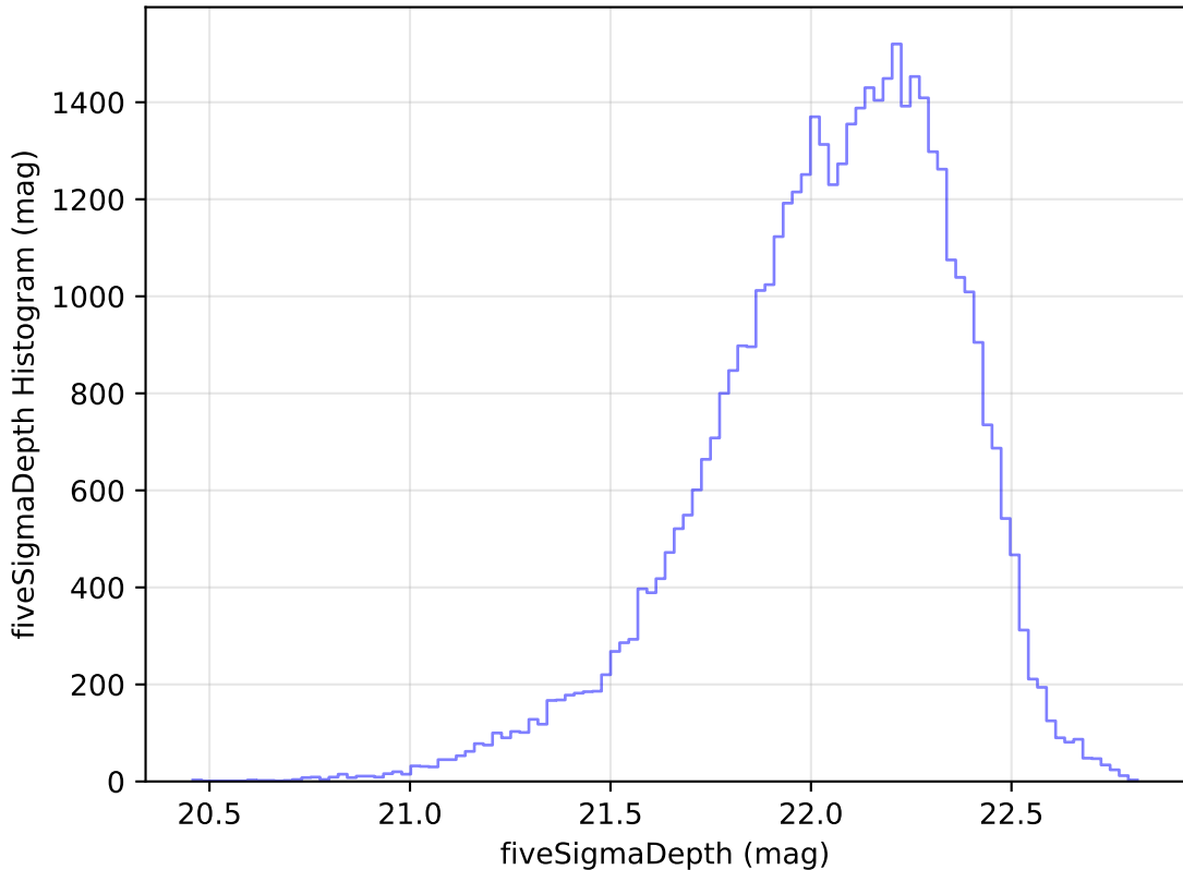
internal_u_expt60_nscale1.5v3.4_10yrs Yr 1 y band: fiveSigmaDepth Histogram
