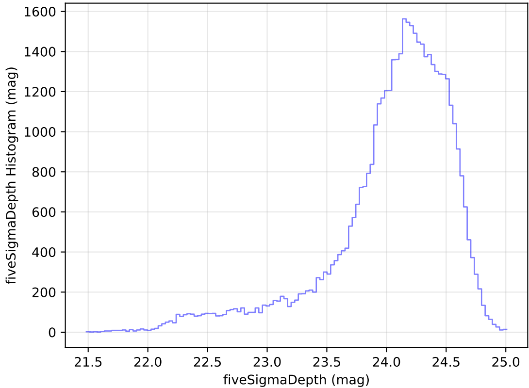
internal_u_expt60_nscale1.5v3.4_10yrs Yr 1 r band: fiveSigmaDepth Histogram
