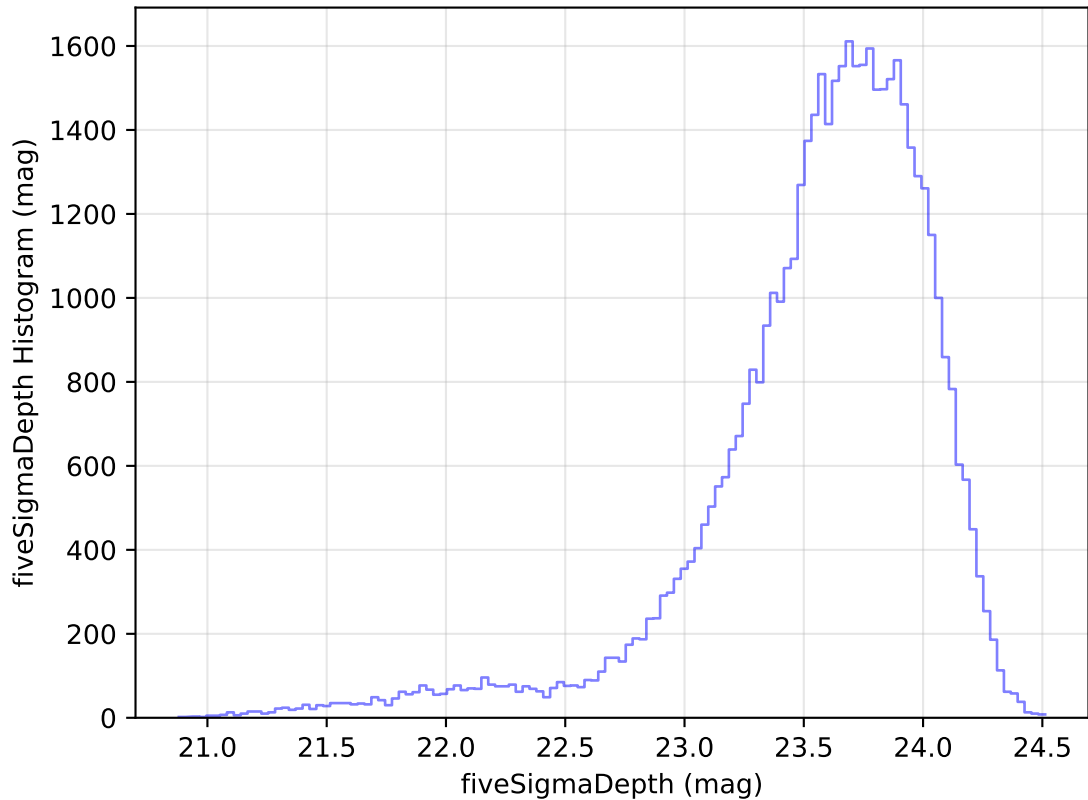
internal_u_expt60_nscale1.5v3.4_10yrs Yr 1 i band: fiveSigmaDepth Histogram
