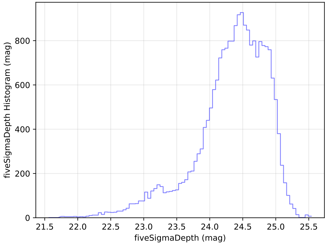
internal_u_expt60_nscale1.5v3.4_10yrs Yr 1 g band: fiveSigmaDepth Histogram
