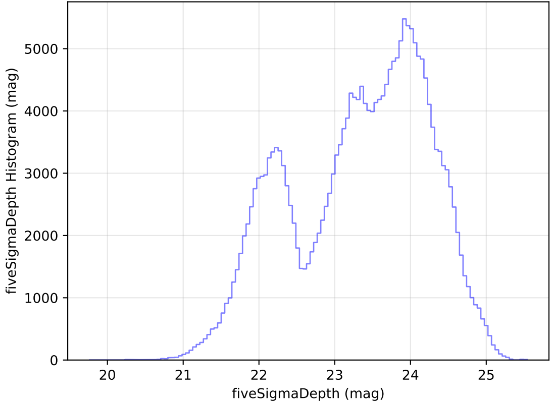
internal_u_expt60_nscale1.5v3.4_10yrs Yr 1 all bands: fiveSigmaDepth Histogram
