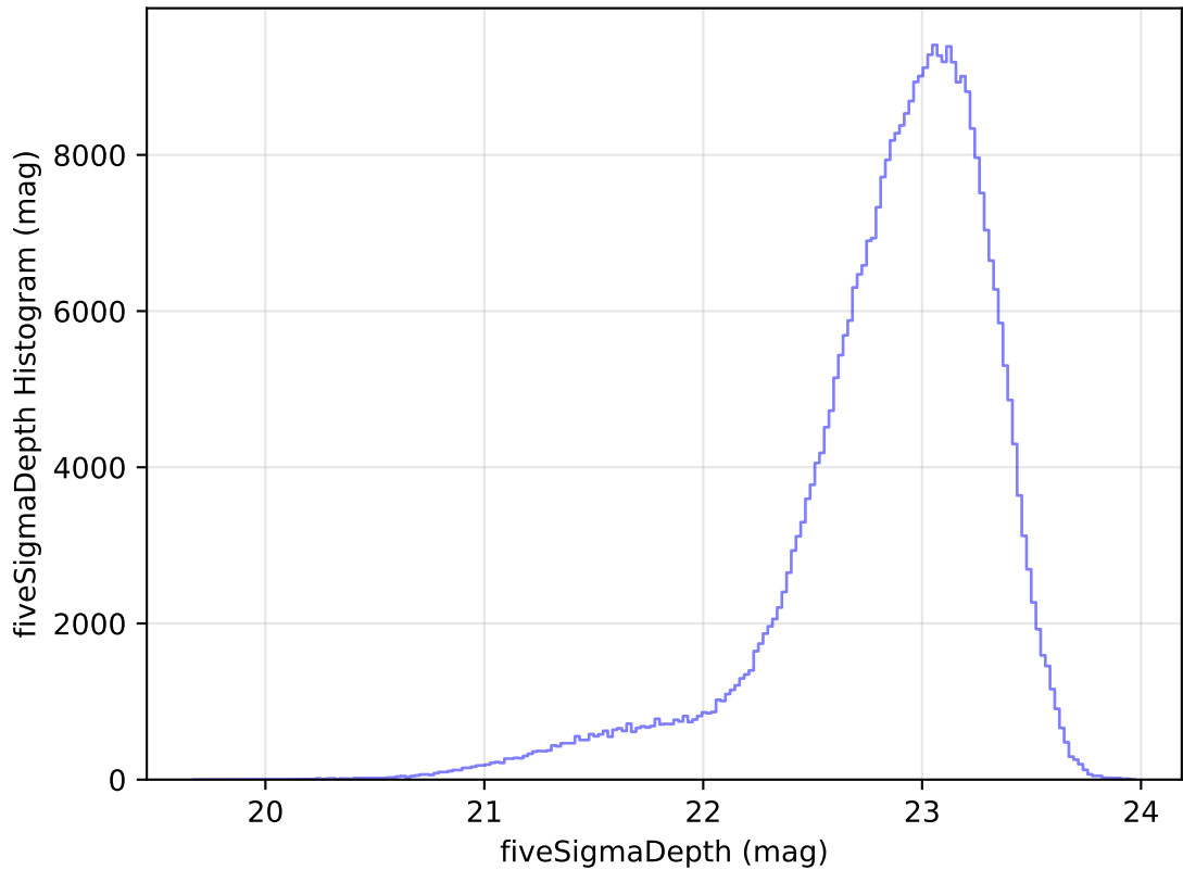
internal_u_expt60_nscale1.5v3.4_10yrs WFD z band: fiveSigmaDepth Histogram
