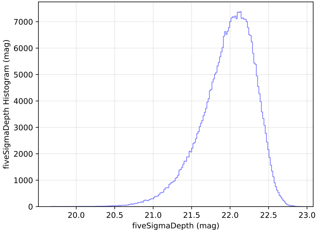
internal_u_expt60_nscale1.5v3.4_10yrs WFD y band: fiveSigmaDepth Histogram
