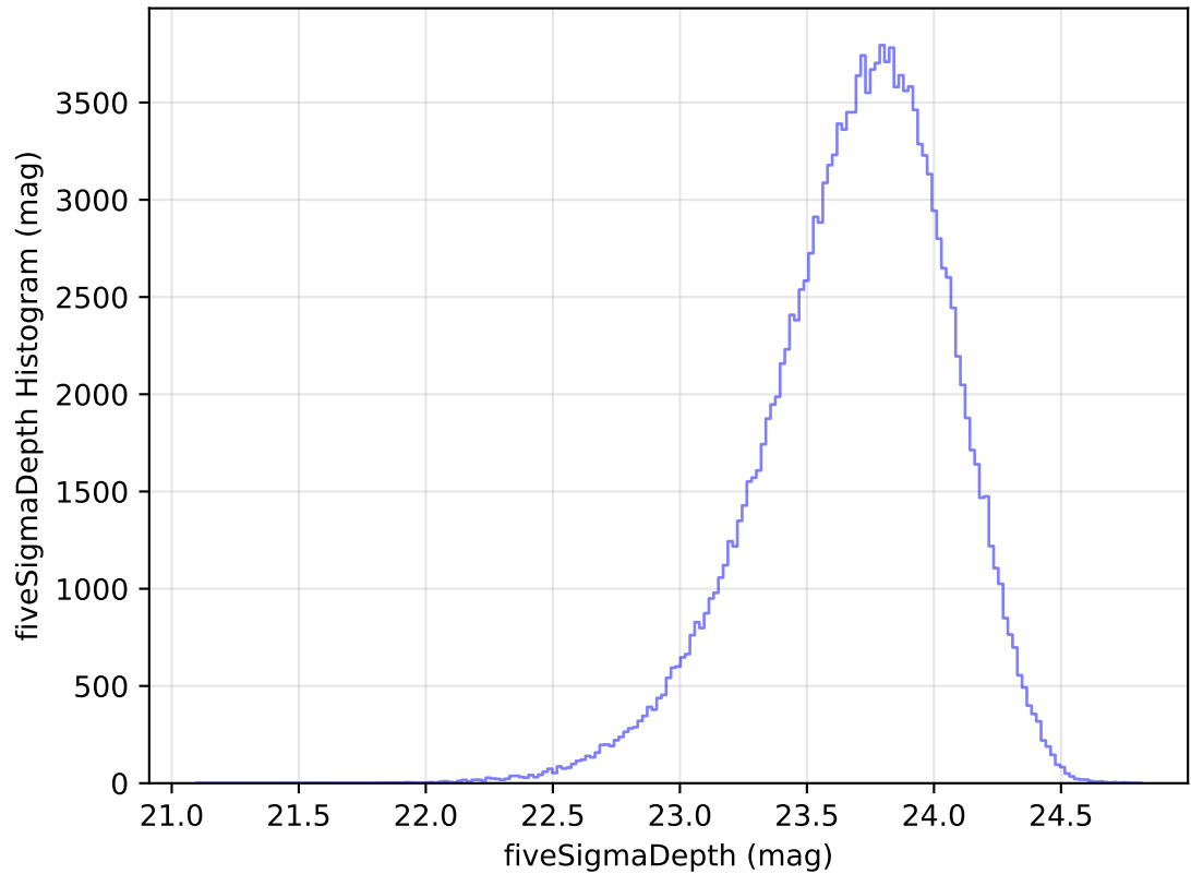
internal_u_expt60_nscale1.5v3.4_10yrs WFD u band: fiveSigmaDepth Histogram
