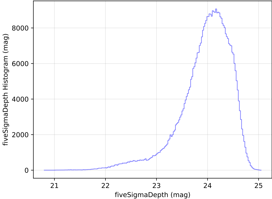
internal_u_expt60_nscale1.5v3.4_10yrs WFD r band: fiveSigmaDepth Histogram
