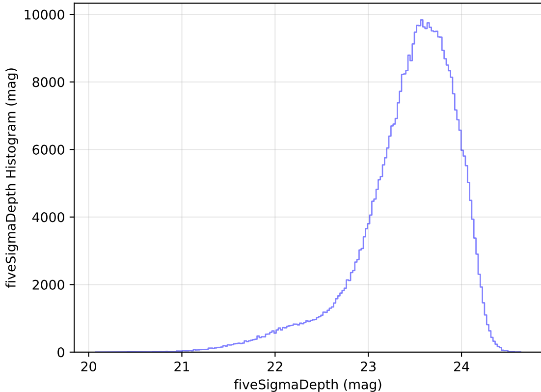
internal_u_expt60_nscale1.5v3.4_10yrs WFD i band: fiveSigmaDepth Histogram
