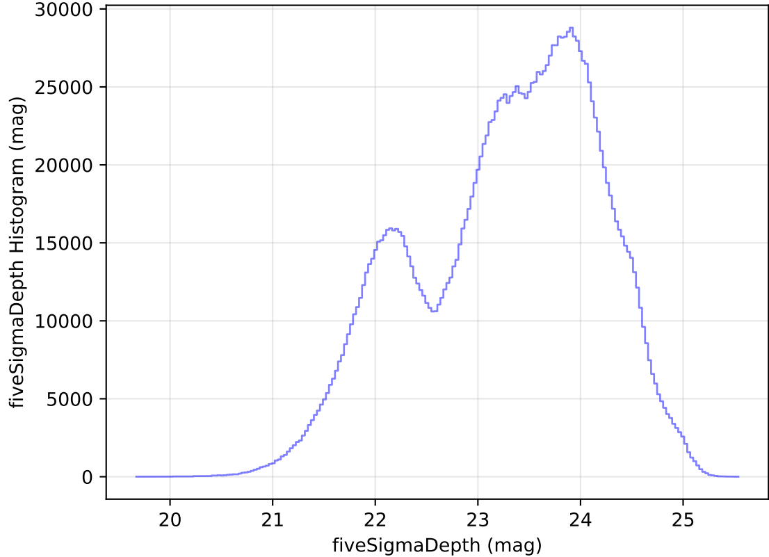
internal_u_expt60_nscale1.5v3.4_10yrs WFD all bands: fiveSigmaDepth Histogram
