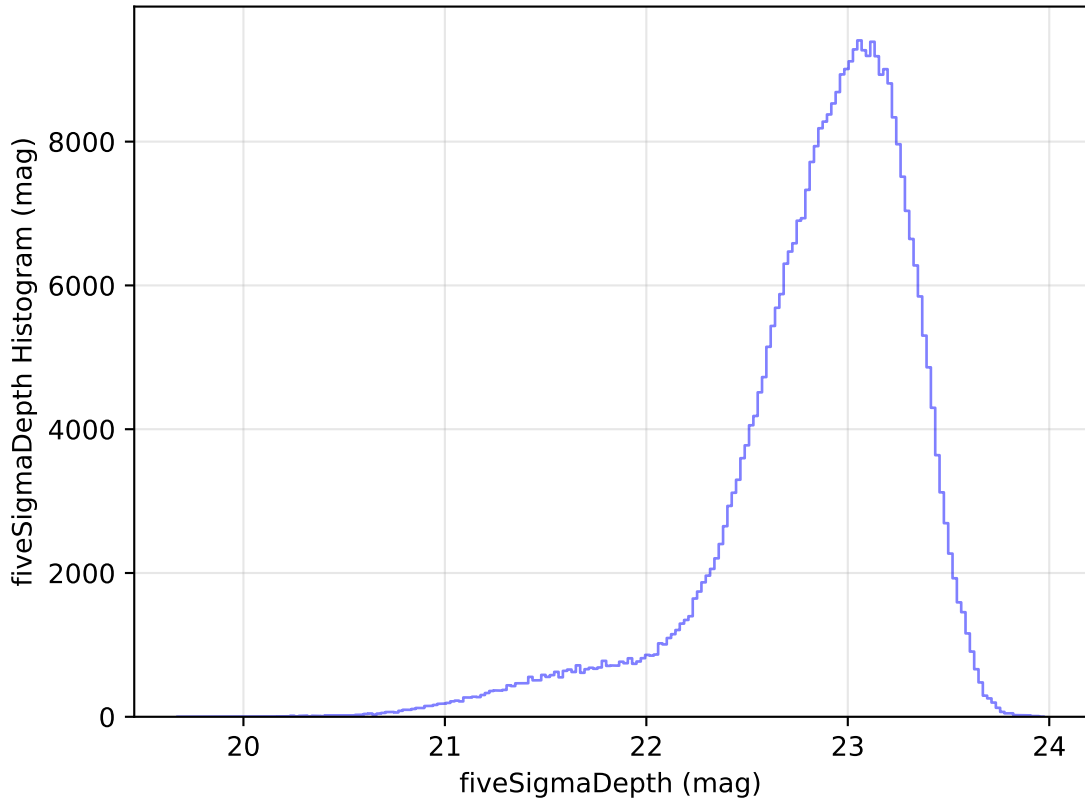
internal_u_expt60_nscale1.5v3.4_10yrs All sky z band: fiveSigmaDepth Histogram
