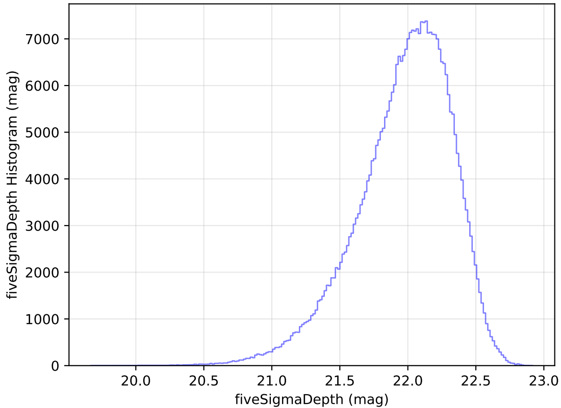
internal_u_expt60_nscale1.5v3.4_10yrs All sky y band: fiveSigmaDepth Histogram
