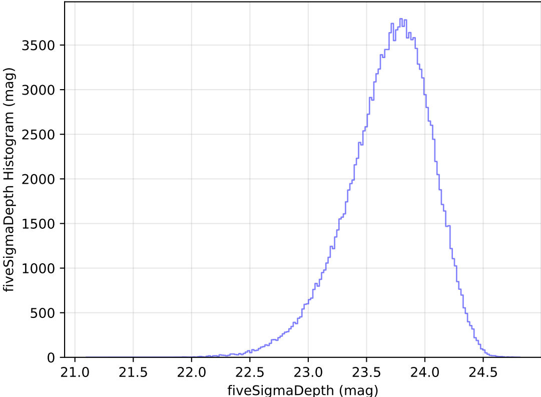
internal_u_expt60_nscale1.5v3.4_10yrs All sky u band: fiveSigmaDepth Histogram
