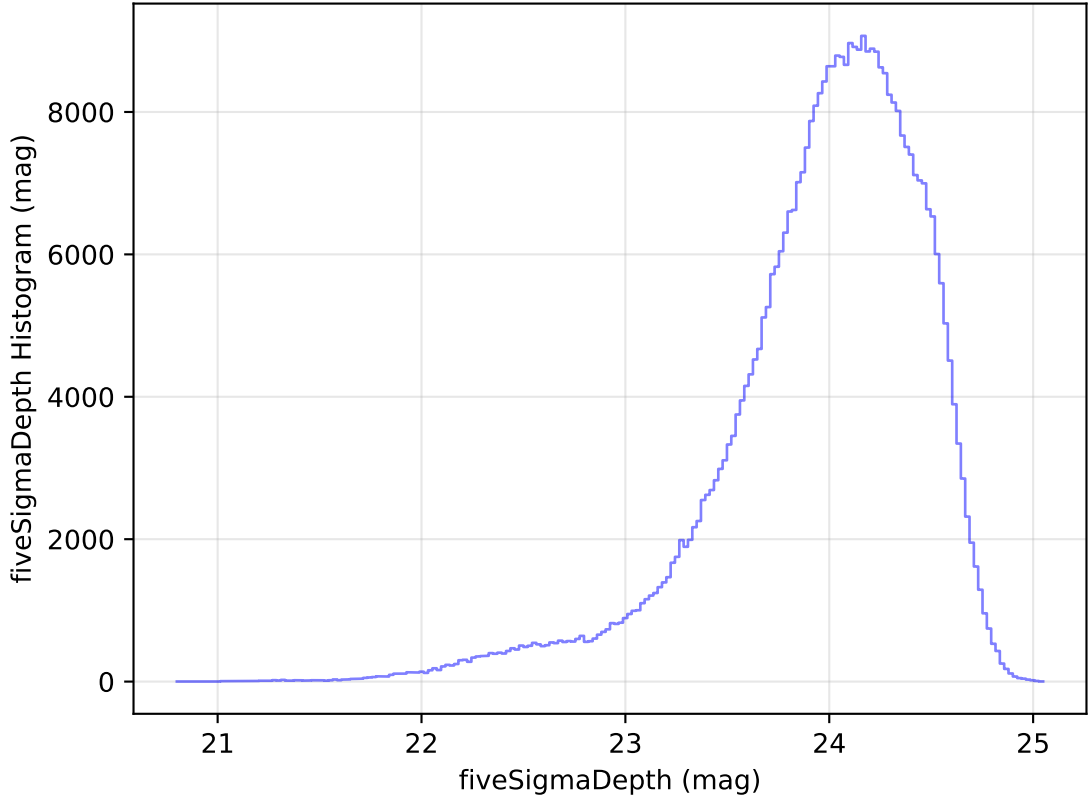
internal_u_expt60_nscale1.5v3.4_10yrs All sky r band: fiveSigmaDepth Histogram
