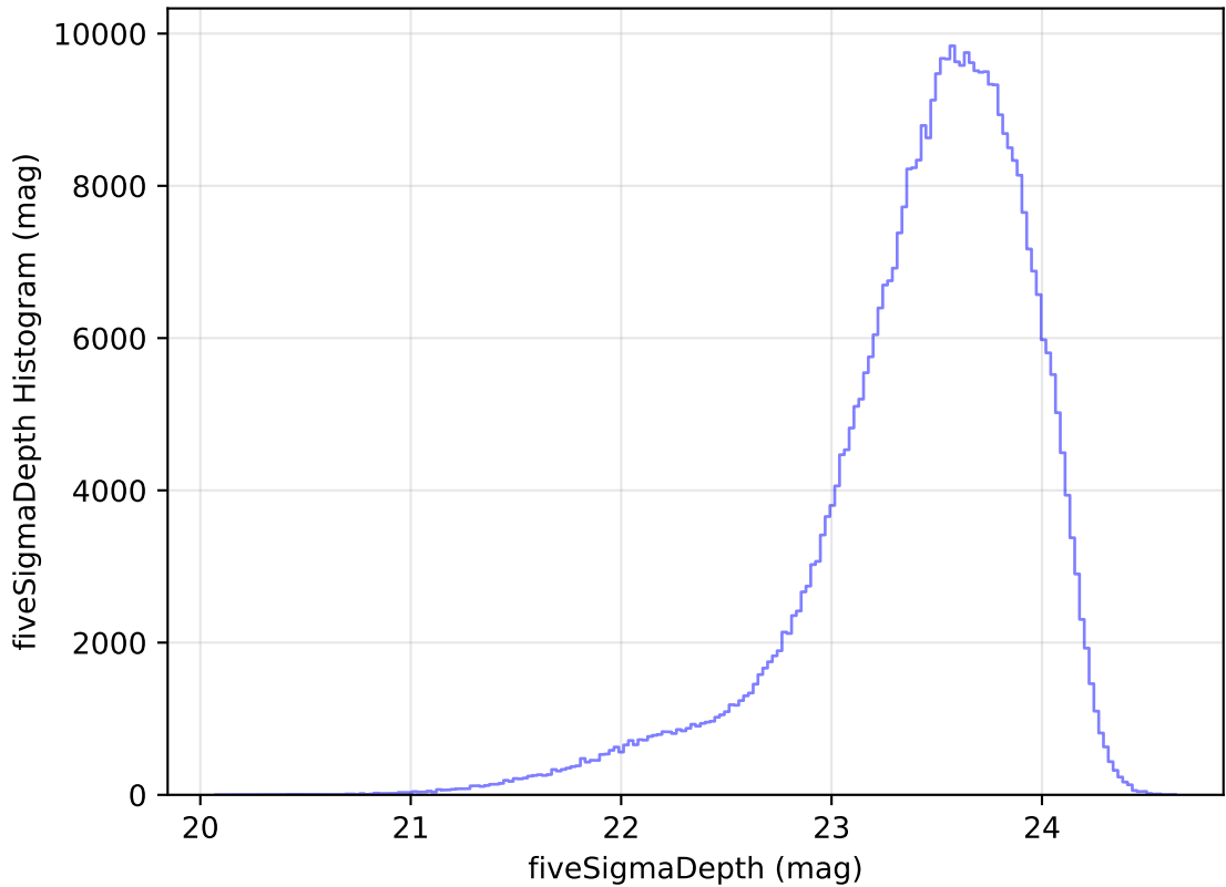
internal_u_expt60_nscale1.5v3.4_10yrs All sky i band: fiveSigmaDepth Histogram
