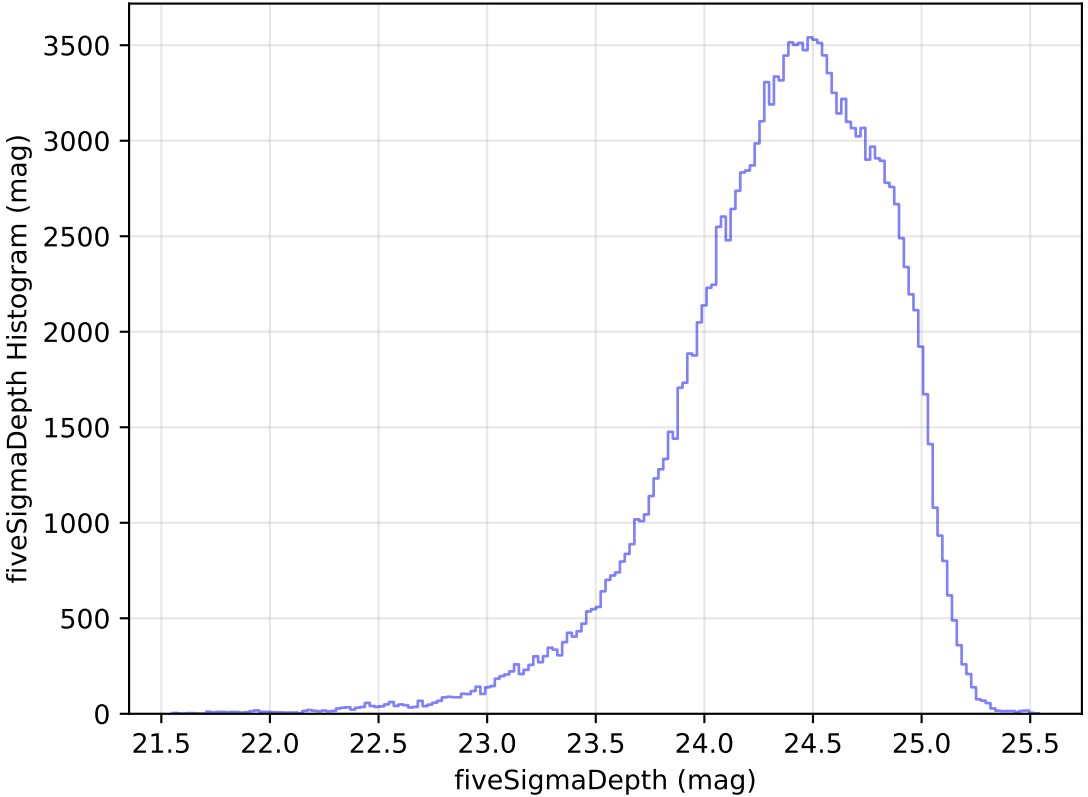
internal_u_expt60_nscale1.5v3.4_10yrs All sky g band: fiveSigmaDepth Histogram
