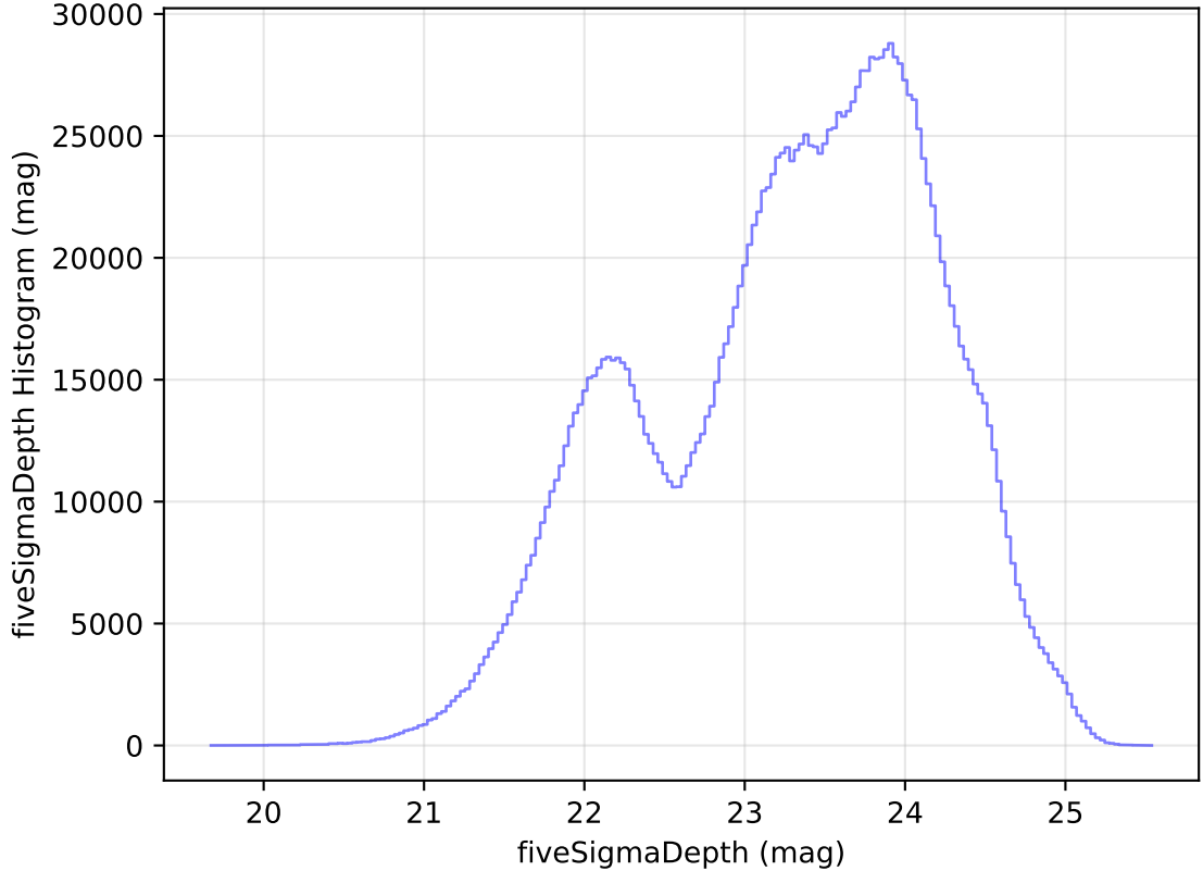
internal_u_expt60_nscale1.5v3.4_10yrs All sky all bands: fiveSigmaDepth Histogram
