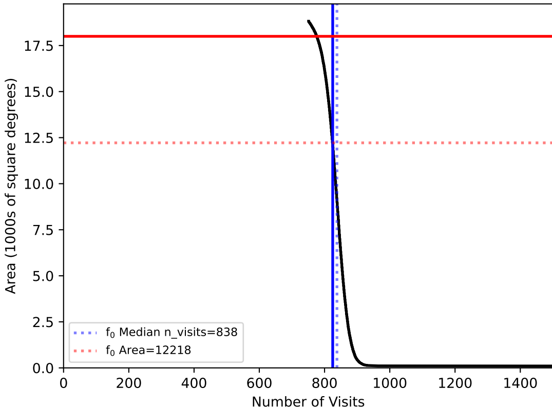
internal_u_expt60_nscale1.5v3.4_10yrs WFD: fO
