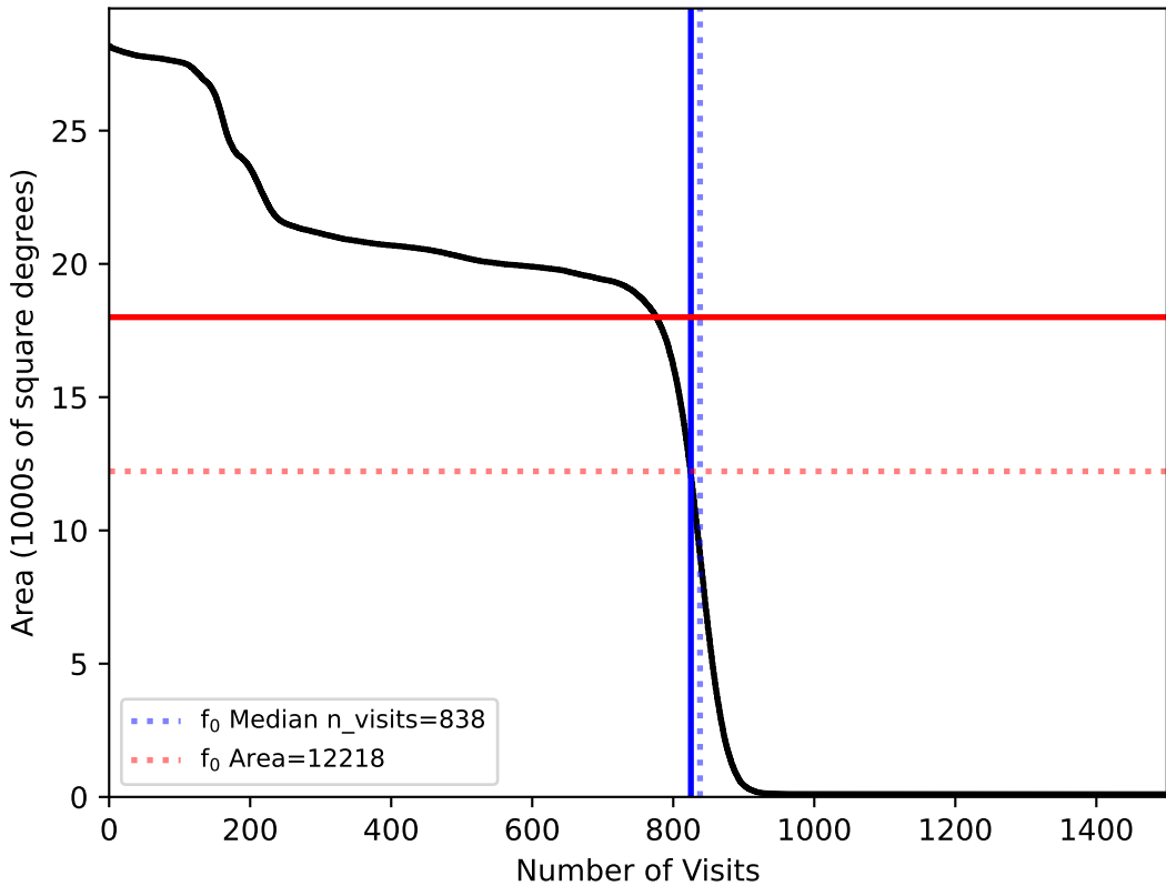
internal_u_expt60_nscale1.5v3.4_10yrs All sky: f0
