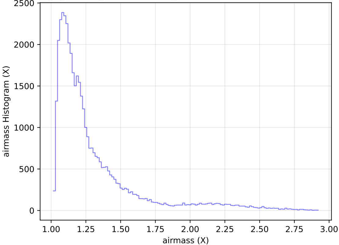
internal_u_expt60_nscale1.5v3.4_10yrs Yr 1 z band: airmass Histogram
