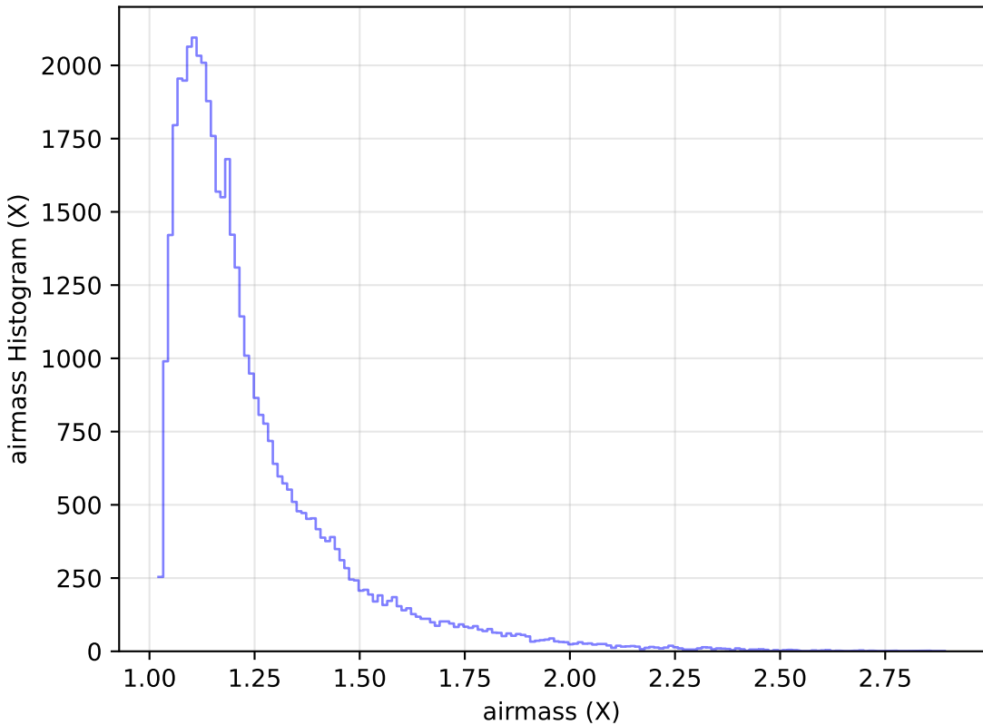
internal_u_expt60_nscale1.5v3.4_10yrs Yr 1 y band: airmass Histogram
