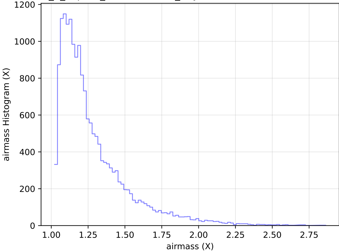
internal_u_expt60_nscale1.5v3.4_10yrs Yr 1 u band: airmass Histogram
