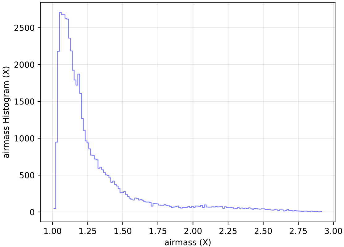
internal_u_expt60_nscale1.5v3.4_10yrs Yr 1 i band: airmass Histogram
