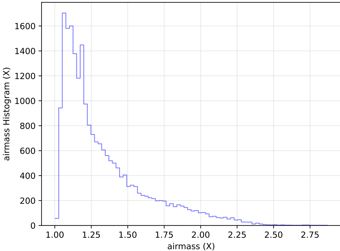
internal_u_expt60_nscale1.5v3.4_10yrs Yr 1 g band: airmass Histogram
