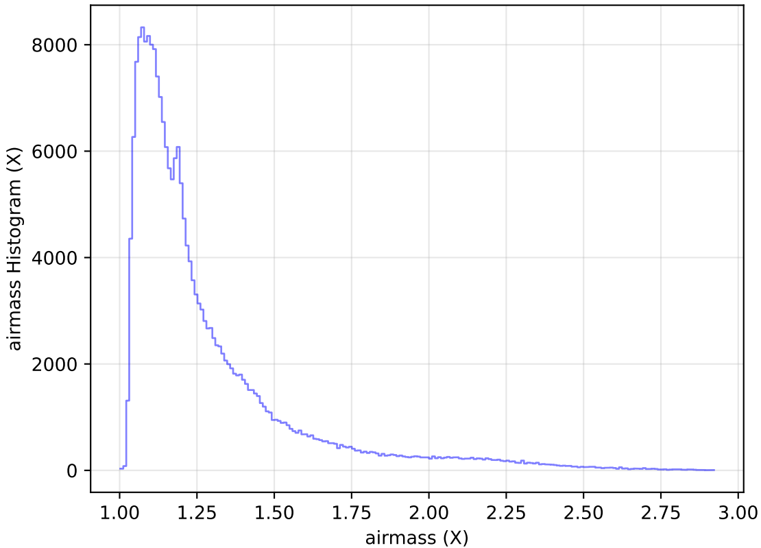
internal_u_expt60_nscale1.5v3.4_10yrs Yr 1 all bands: airmass Histogram
