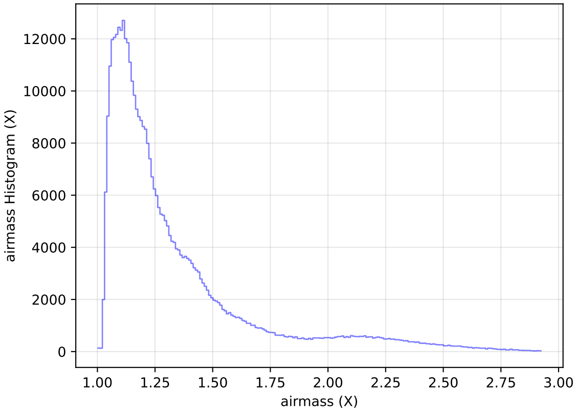
internal_u_expt60_nscale1.5v3.4_10yrs WFD z band: airmass Histogram
