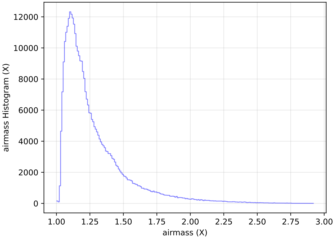
internal_u_expt60_nscale1.5v3.4_10yrs WFD y band: airmass Histogram
