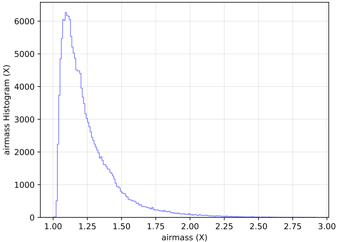
internal_u_expt60_nscale1.5v3.4_10yrs WFD u band: airmass Histogram
