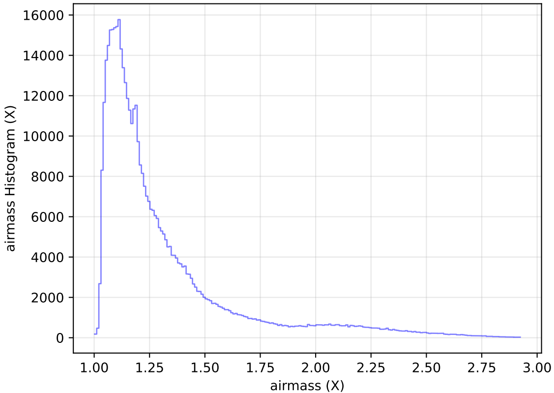
internal_u_expt60_nscale1.5v3.4_10yrs WFD i band: airmass Histogram
