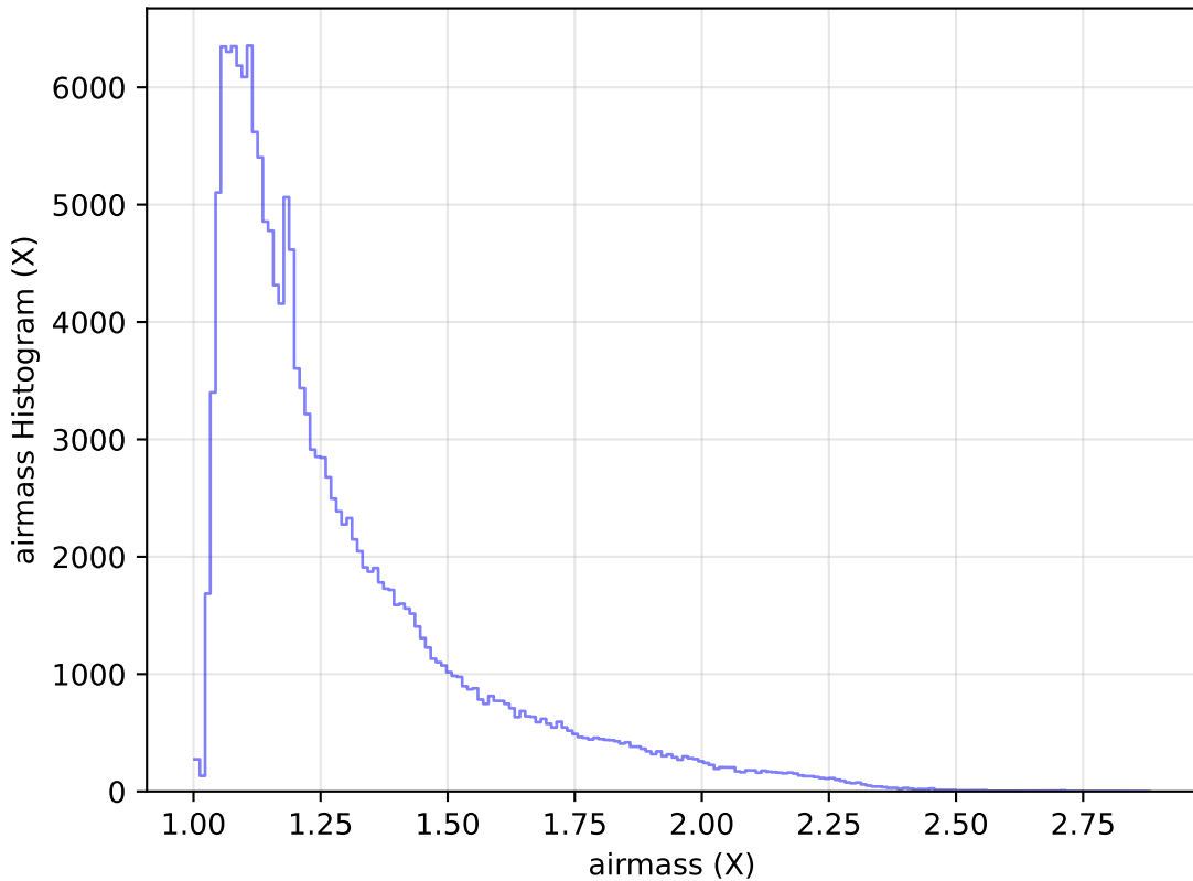
internal_u_expt60_nscale1.5v3.4_10yrs WFD g band: airmass Histogram
