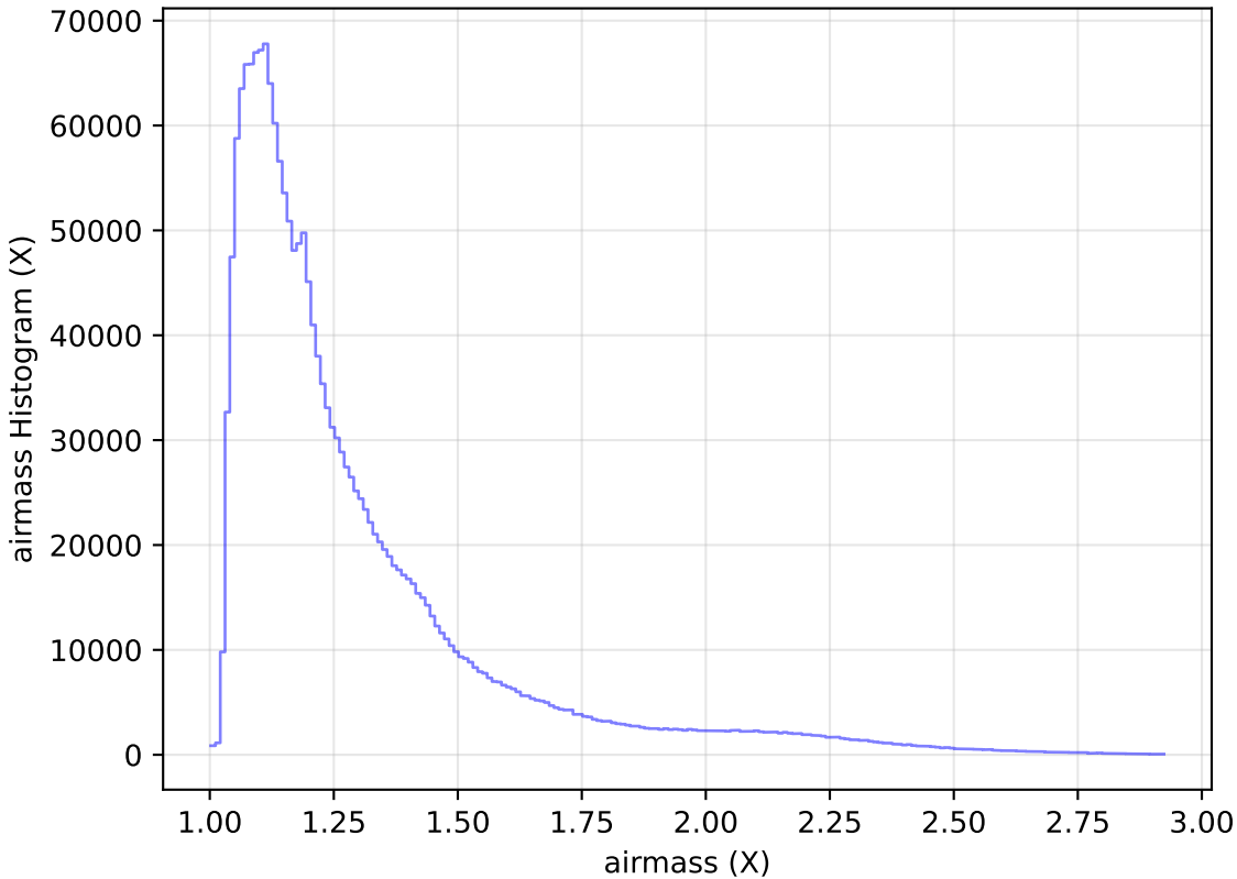
internal_u_expt60_nscale1.5v3.4_10yrs WFD all bands: airmass Histogram
