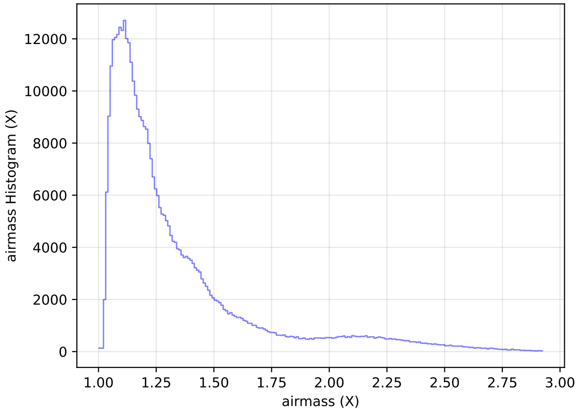
internal_u_expt60_nscale1.5v3.4_10yrs All sky z band: airmass Histogram
