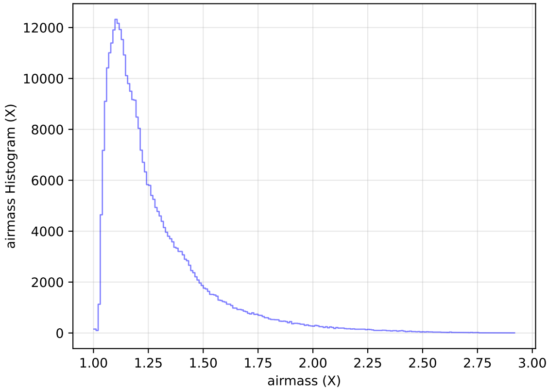
internal_u_expt60_nscale1.5v3.4_10yrs All sky y band: airmass Histogram
