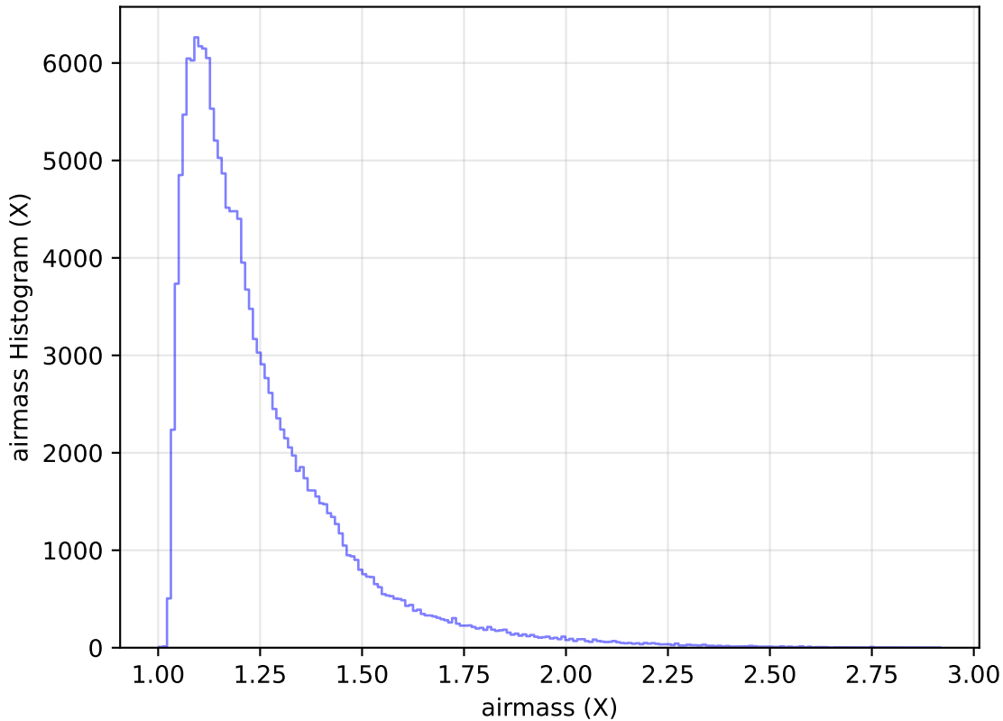
internal_u_expt60_nscale1.5v3.4_10yrs All sky u band: airmass Histogram
