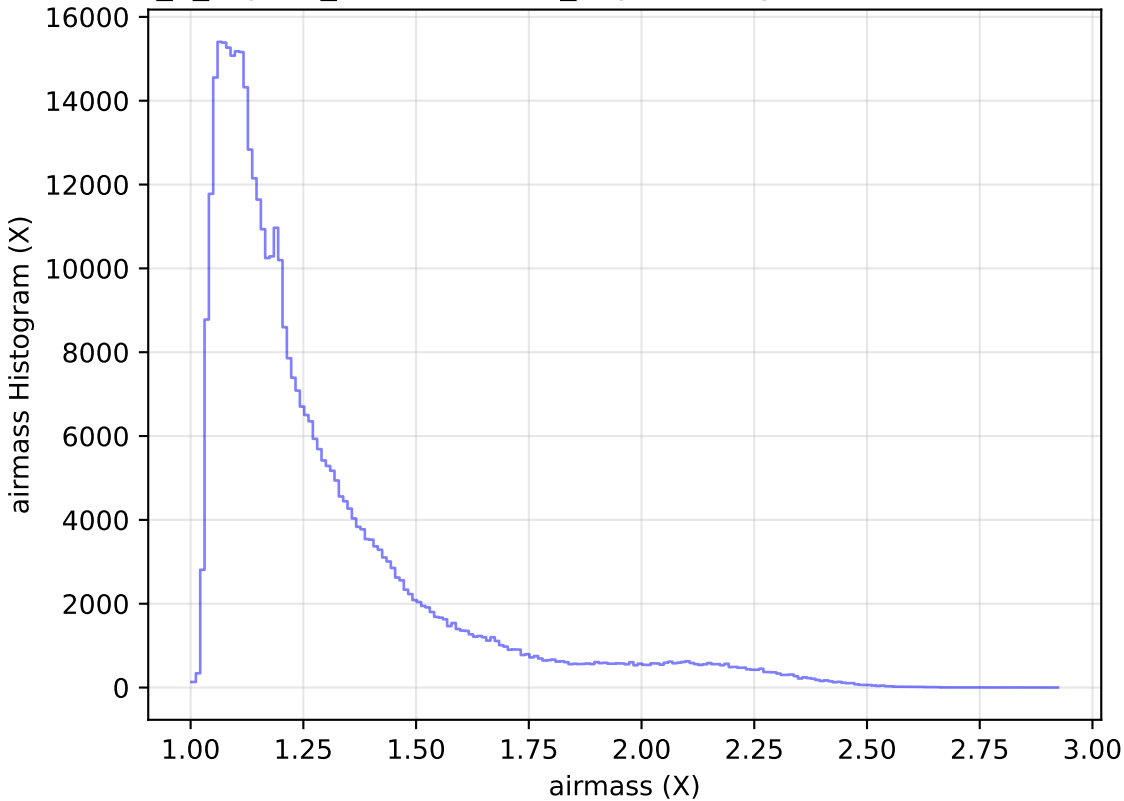
internal_u_expt60_nscale1.5v3.4_10yrs All sky r band: airmass Histogram
