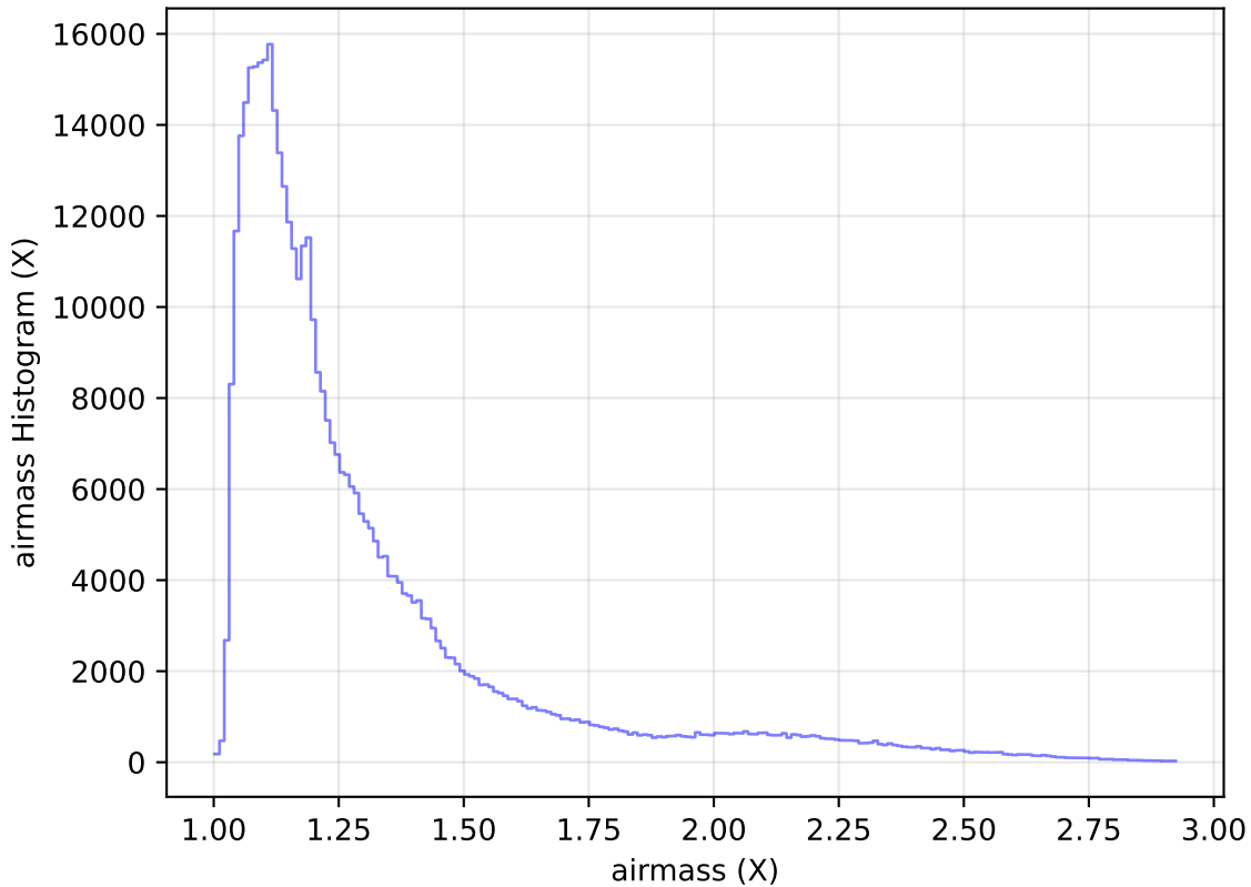
internal_u_expt60_nscale1.5v3.4_10yrs All sky i band: airmass Histogram
