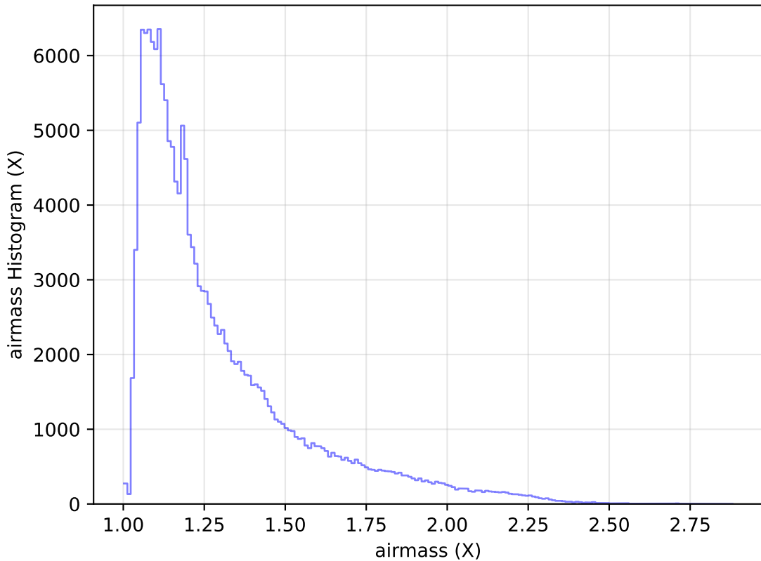
internal_u_expt60_nscale1.5v3.4_10yrs All sky g band: airmass Histogram
