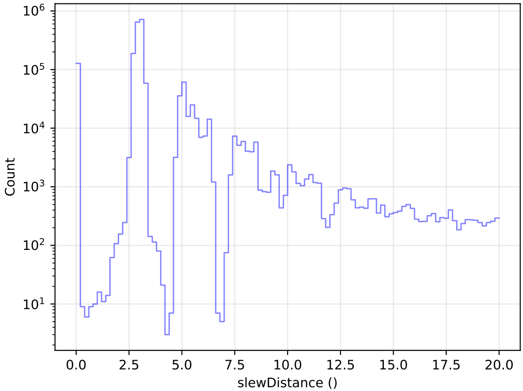
internal_u_expt60_nscale1.5v3.4_10yrs All visits: Zoom Slew Distance Histogram
