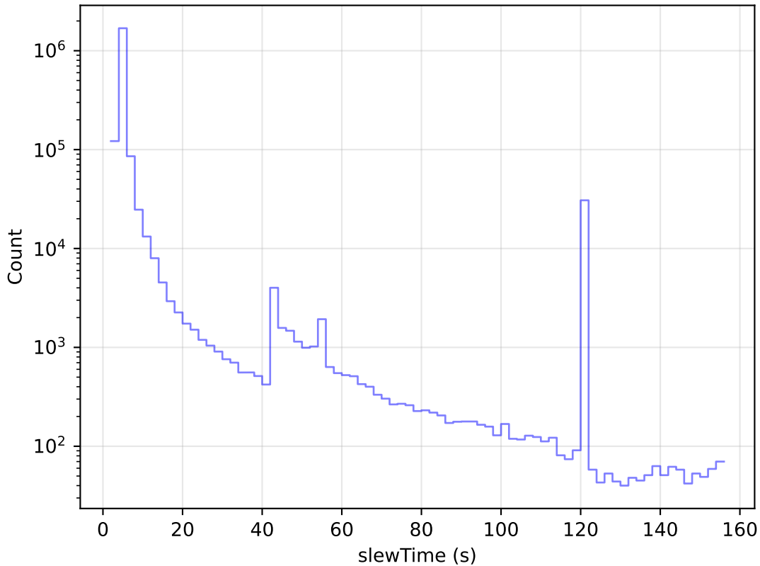
internal_u_expt60_nscale1.5v3.4_10yrs All visits: Slew Time Histogram
