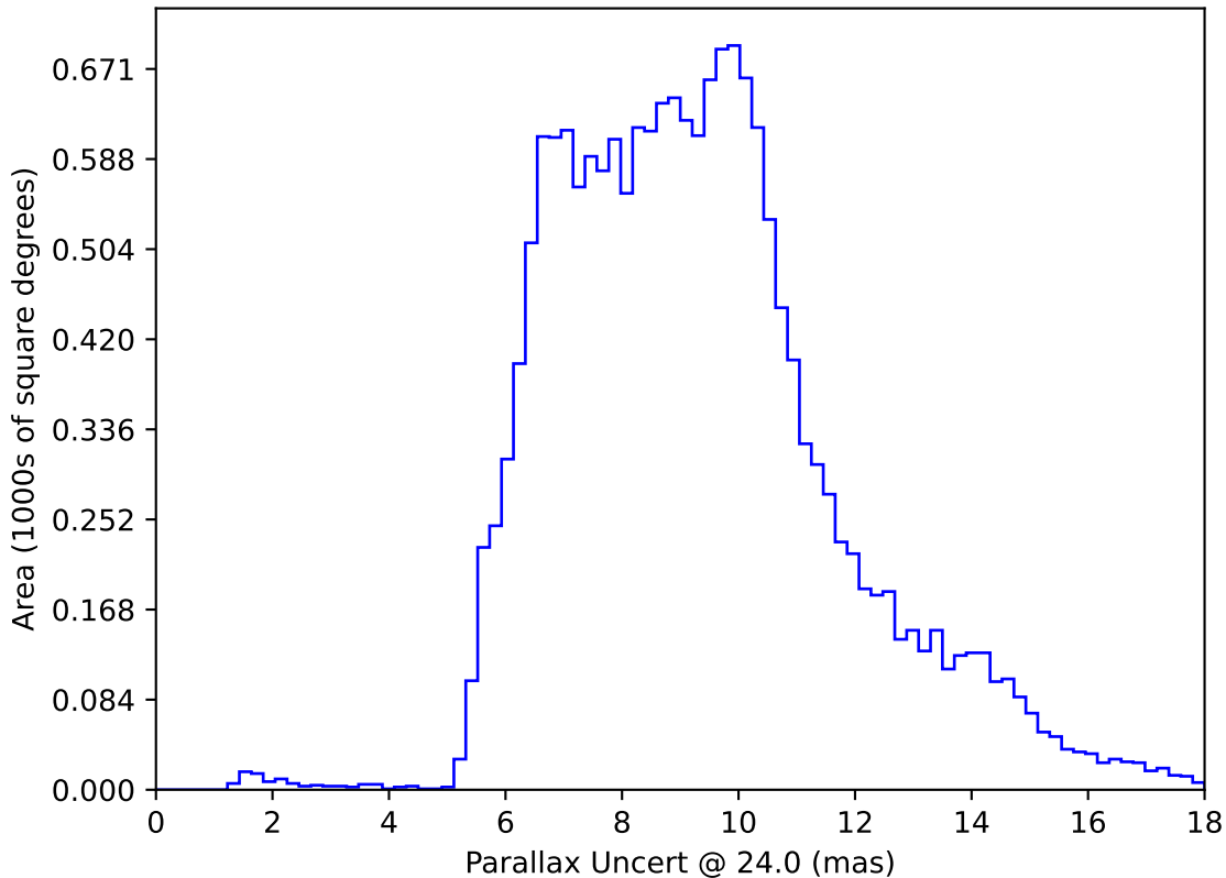
internal_u_expt60_nscale1.5v3.4_10yrs WFD: Parallax Uncert @ 24.0
